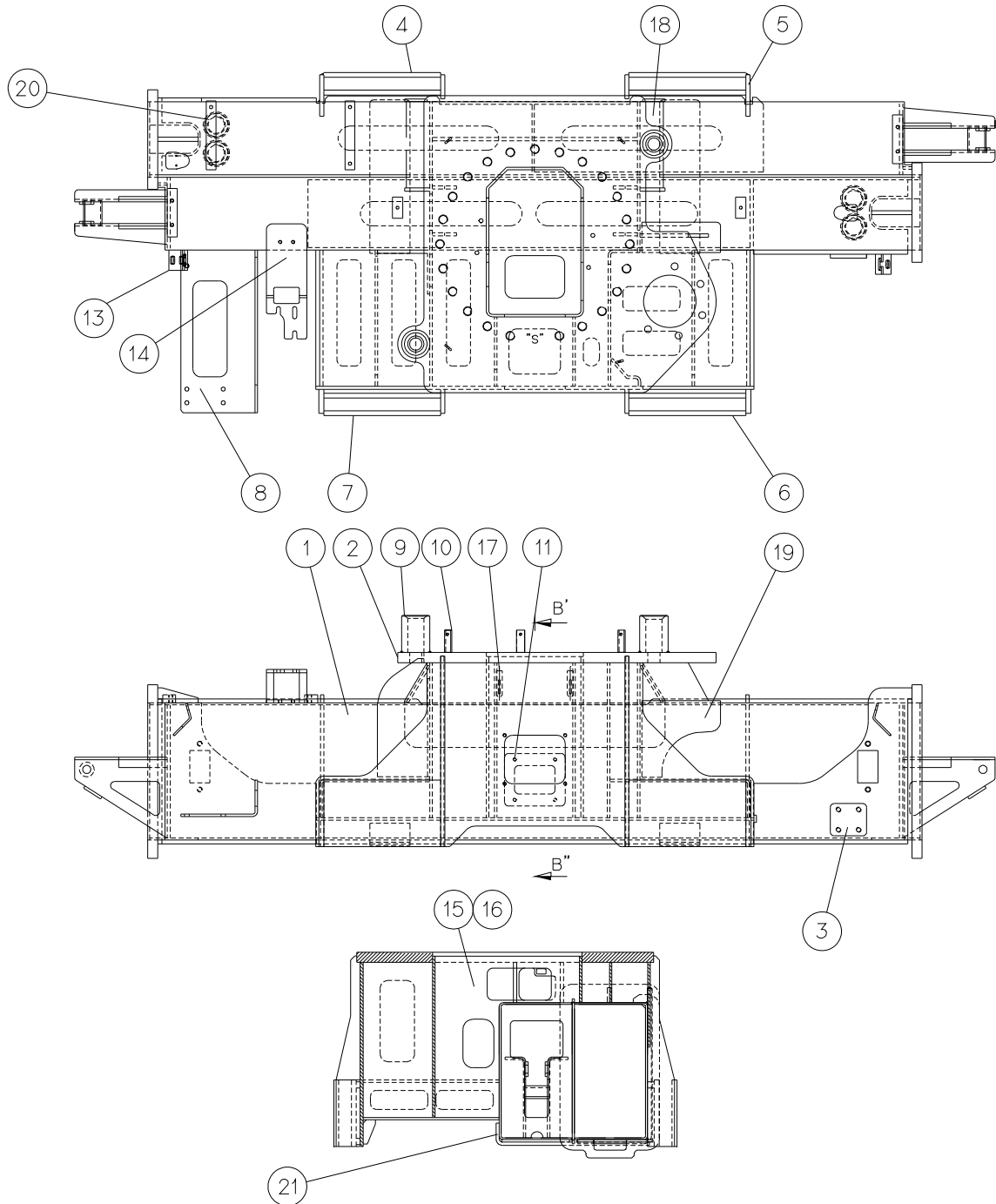
SECTION B'-B''
